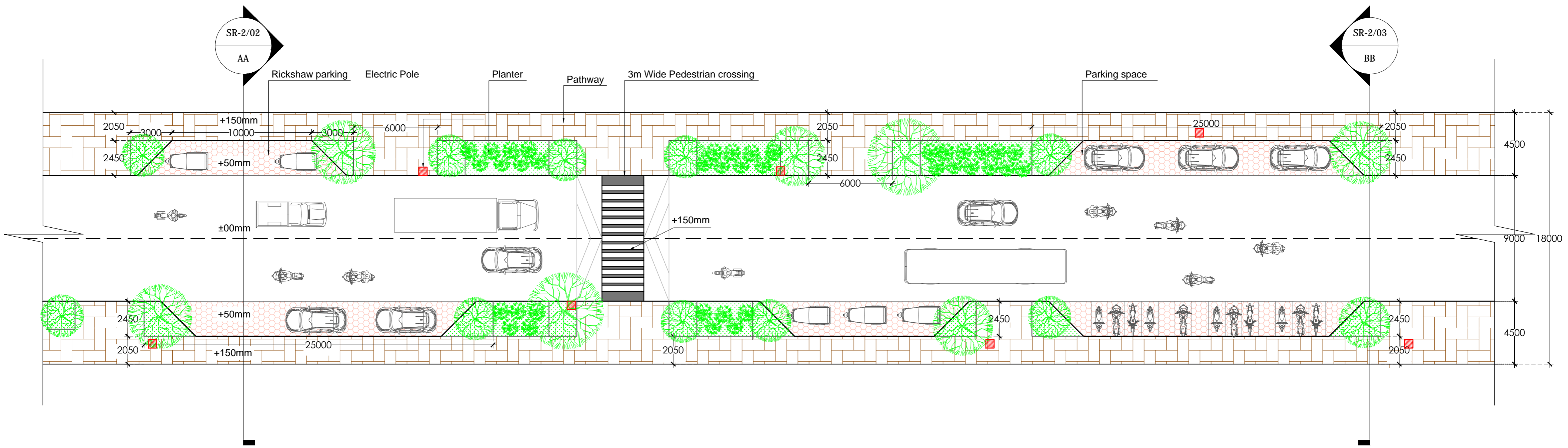
⊕ 18 m Wide road plan Scale- 1:200
